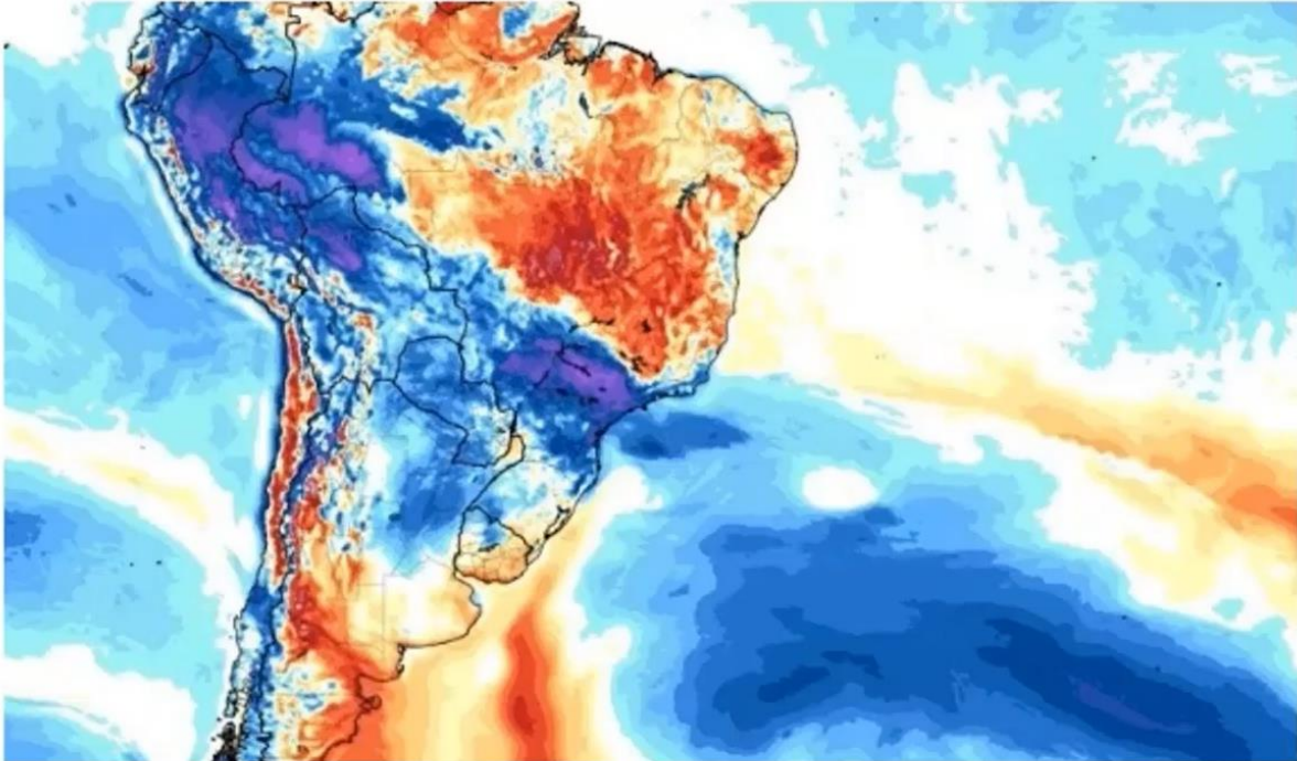
GFS TEMP ANOMALY for JULY 18
