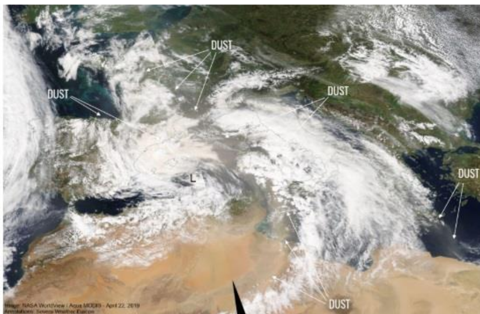
NASA Aqua satellite made this image of the broad cutoff low pushing Saharan dust across the Mediterranean into Europe today, April 22, 2019 around local noon. Note the thick band of dust pushing across the southern Mediterranean between Tunisia, Malta and Sicily, across the Tyrrhenian sea,
