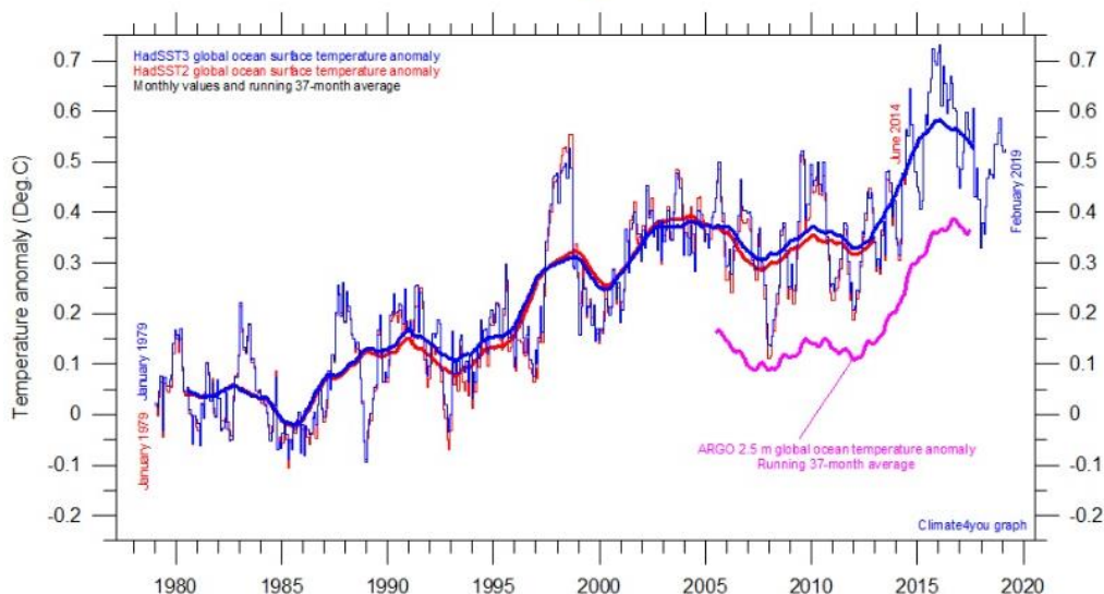
Global monthly average sea surface temperature (SST) since 1979 according to University of East Anglia's Climatic Research Unit (CRU) , UK. The data series (HadSST2) are described by Ranier et al. (2006) . Base period: 1961-1990. The thick line is the simple running 37 month average, nearly corresponding to a running 3 yr average. Magenta line is the running 37-month average of Argo float measurements, shifted +0.2 degrees for easy comparison. Last month shown: February 2019. Last diagram update: 30 March 2019.
