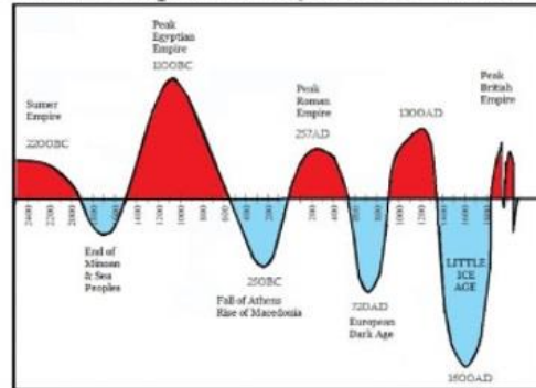
Global Temperatures (2500BC - 2015AD)
