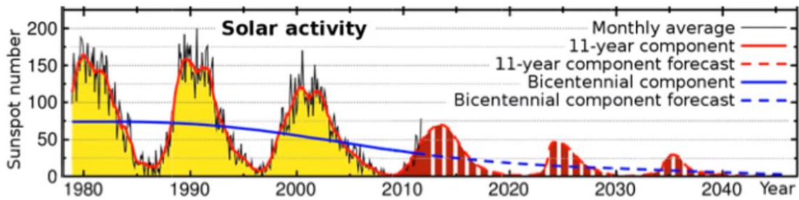
Figure 3. Variations of both the TSI and solar activity in 1978-2011 and a forecast of their variations in cycles 24-26 (up to the year 2045)
