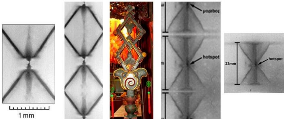
Zeta Pinch (Z-Pinch) Plasma Laboratory Experiments
